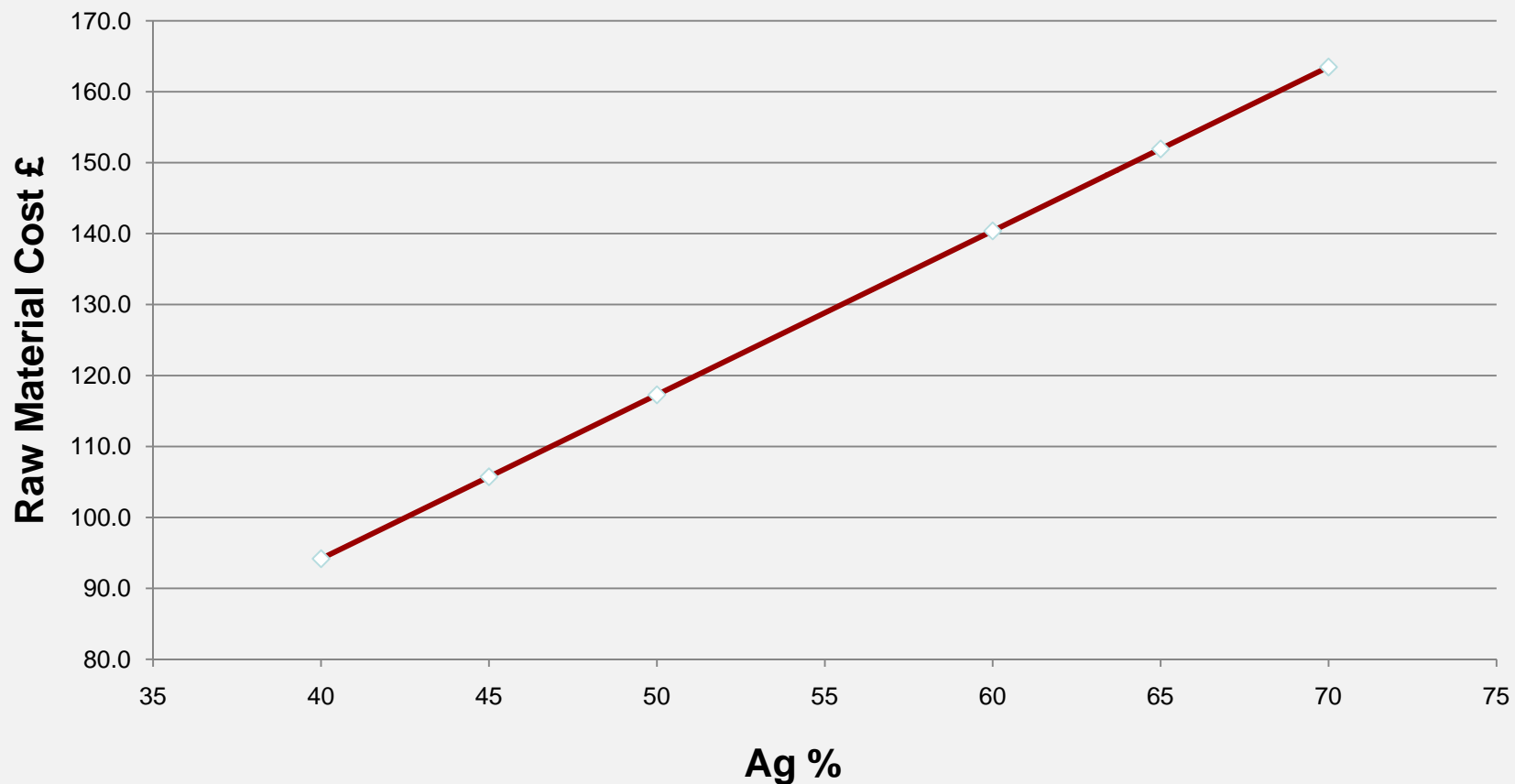
RM costs of flexible silver inks
